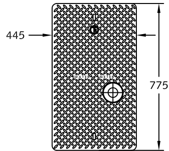
Cast Iron Cover (Reading Hole Optional)
